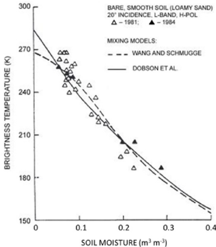
Figure 3.2: L-band brightness temperature response for a bare, smooth soil surface as a function of soil moisture. Soil moisture can range from close to 0.02 \text{ m}^3 \text{ m}^{-3} (very dry), to about 0.40 \text{ m}^3 \text{ m}^{-3} (near saturation for the soil studied). As soil moisture increases the brightness temperature decreases, changing by about 100 K over the full range of soil moisture. Current microwave radiometers have a precision of about 1 K. Details of theoretical modeling and experimental verification for radiometer and radar measurements of vegetation-covered soils can be found in the literature (e.g., Fung et al., 1986; SMAP Handbook, SMAP ATBD, SMOS ATBD).
