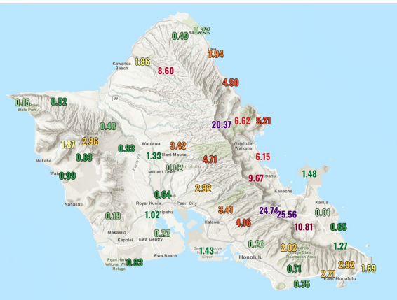
Multi-day rainfall accumulations associated with a severe storm event impacting the windward side of Oahu in late February 2026 (2/20-2/22).
